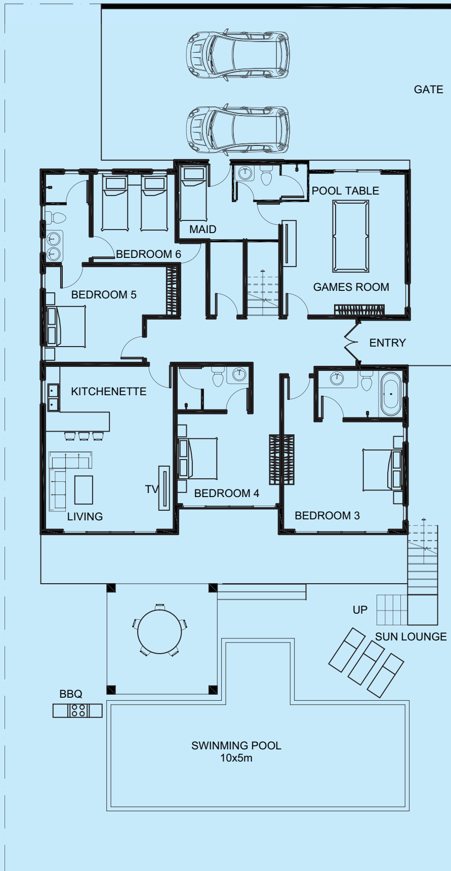
EMERALD LOWER LEVEL FLOOR PLAN
